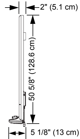
Wall-Mounted Side View
