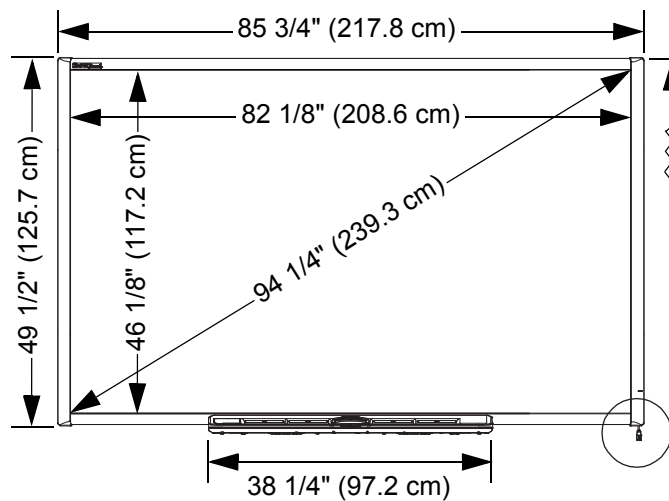
Wall-Mounted Front View
